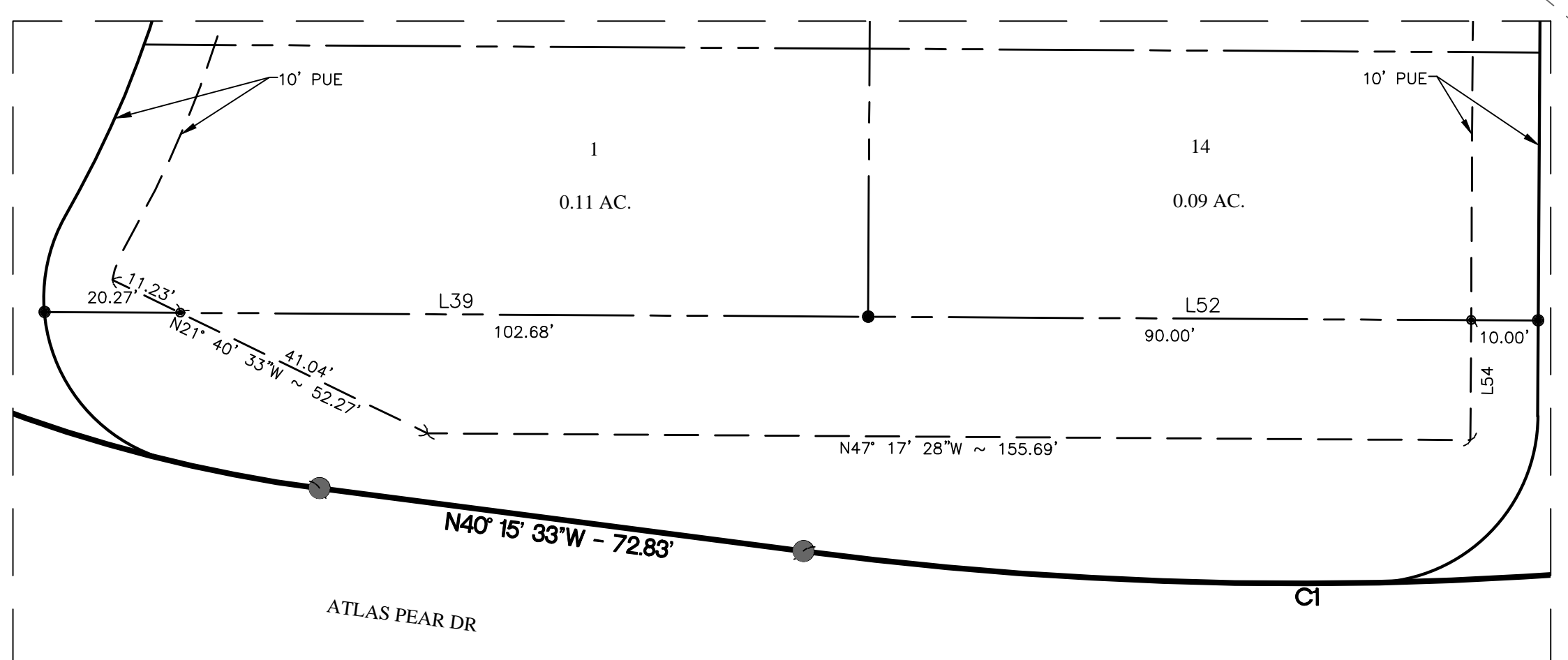
INSET "B" 1"=20'
